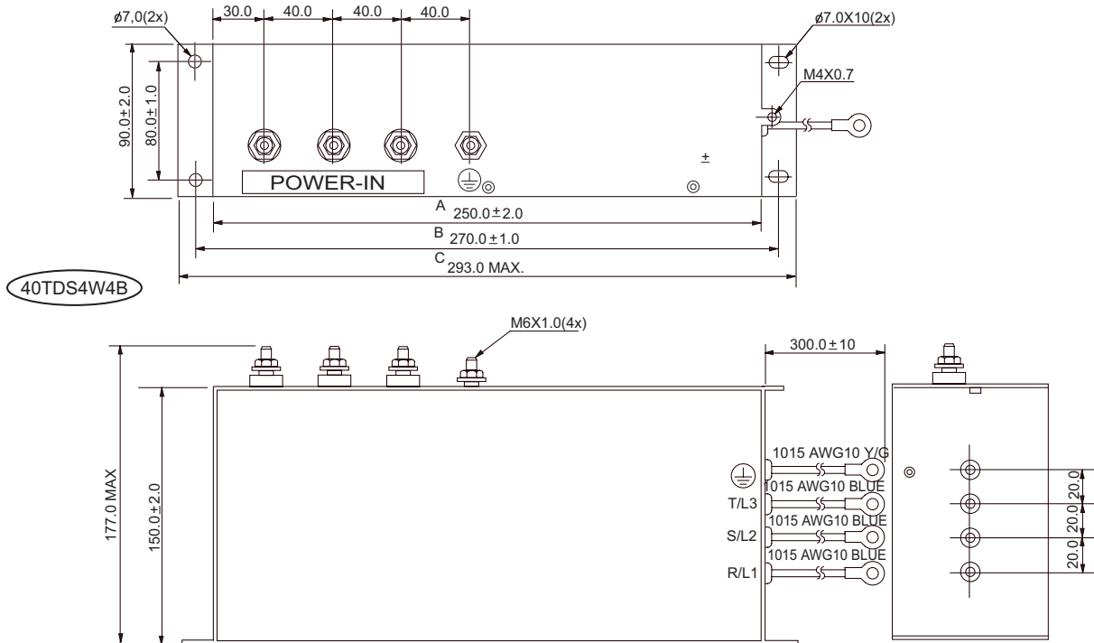
Figure 5 [units = mm]
